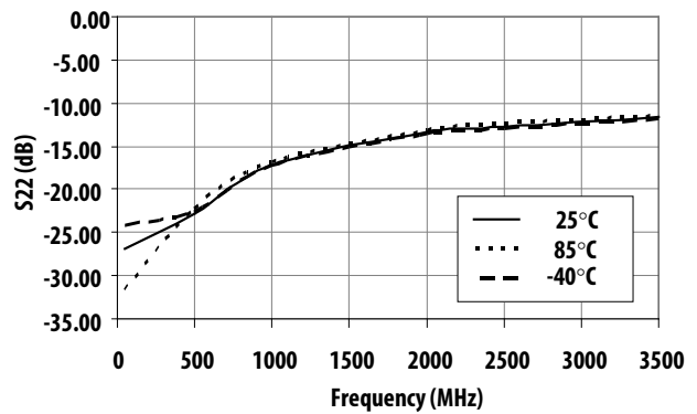
Figure 22. S22 (Return Loss) at Vctrl =5V vs Frequency vs Temperature
