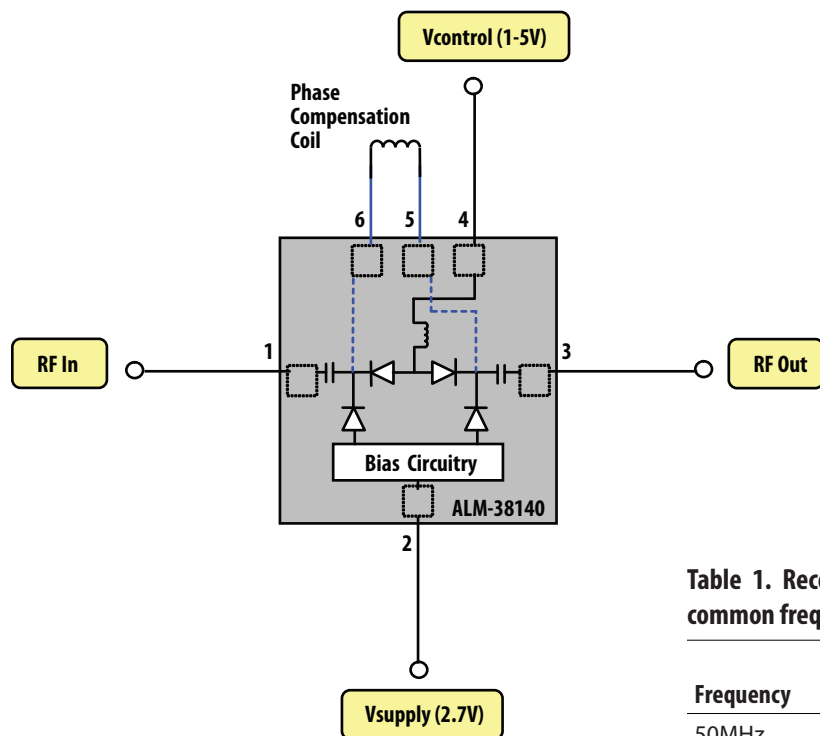
Figure 33. Simplified Schematic
