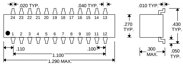
Commercial Gull-Wing (PDU14F-xxA4)
