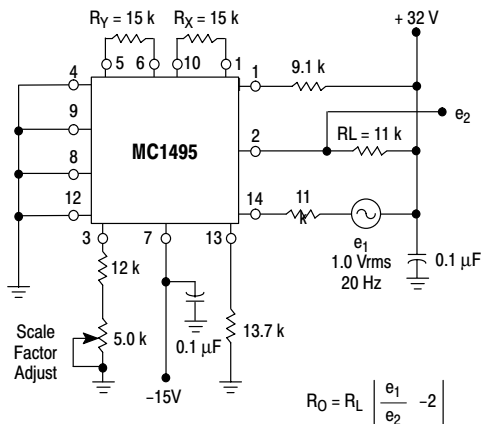
Figure 8. Output Resistance
