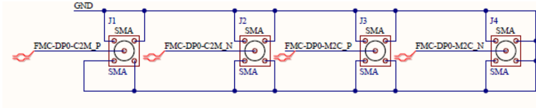
Figure 6. SMA Schematics
