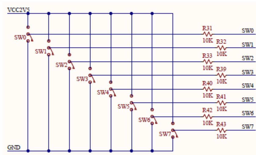
Figure 2. Slide Switch Schematics
