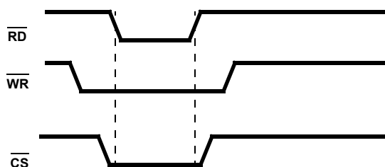
FIGURE 30. READ CYCLE
