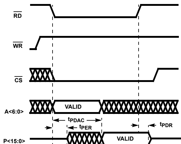
FIGURE 27. MICROPROCESSOR READ TIMING (RDMODE = 0)
