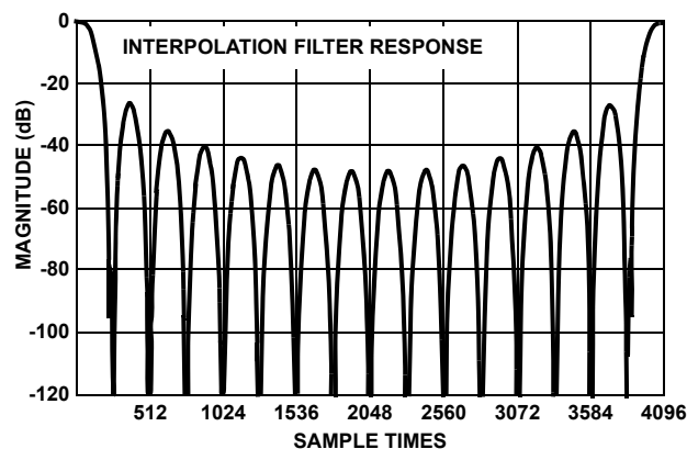
FIGURE 13A. INTERPOLATION FILTER IMPULSE RESPONSE L = 16; FOUT = 4096
