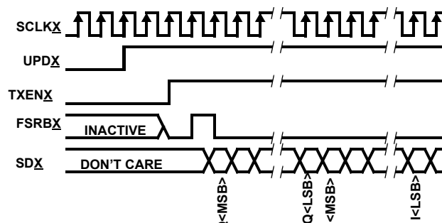
FIGURE 2. SERIAL DATA TRANSFER
