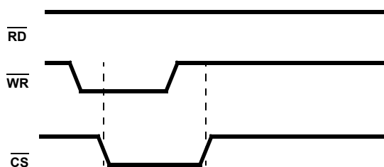
FIGURE 31. WRITE CYCLE
