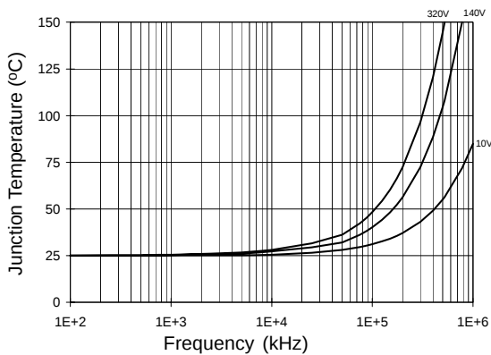
Figure 33. IRS2110S/IRS2113S T_J vs. Frequency (IRFBC30) R_{GATE} = 22 \Omega , V_{CC} = 15 V
