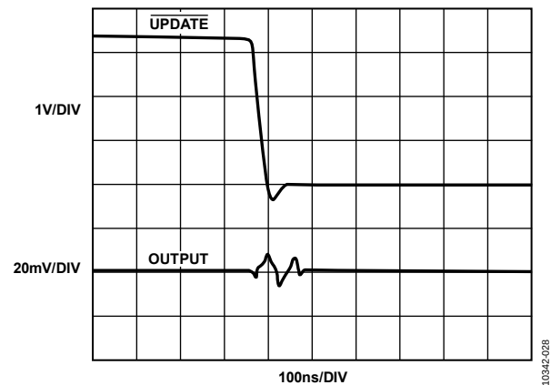
Figure 23. Switching Transient
