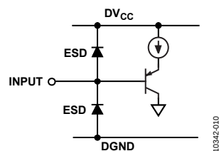
Figure 27. Logic Input
