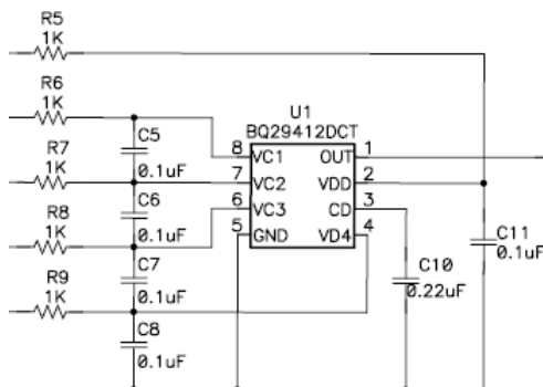
Figure 22. bq29705 Cell Inputs and Time-Delay Capacitor
