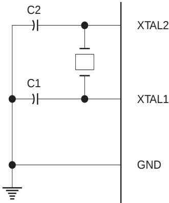
Figure 7. Oscillator Connections
