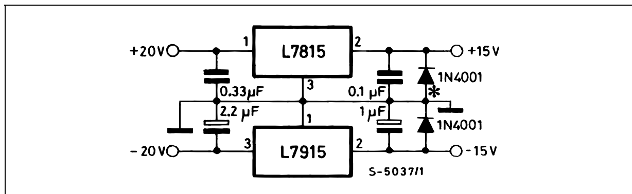
Figure 2 : Split Power Supply ( \pm 15\text{V}/1\text{A} )
