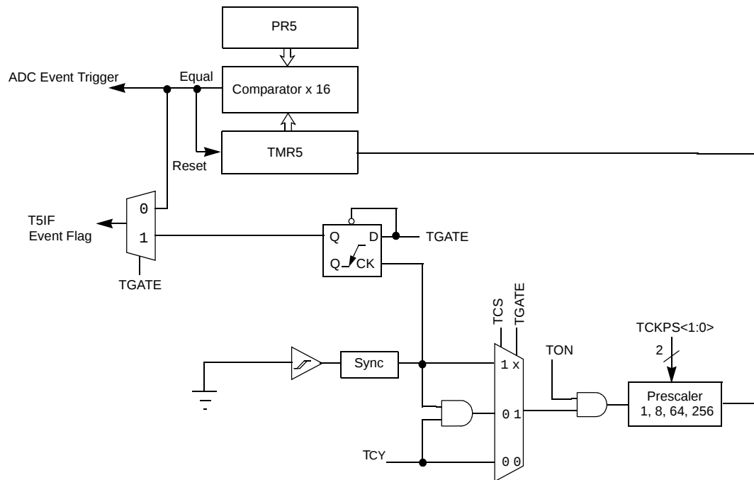
FIGURE 11-3: 16-BIT TIMER5 BLOCK DIAGRAM (TYPE C TIMER)
