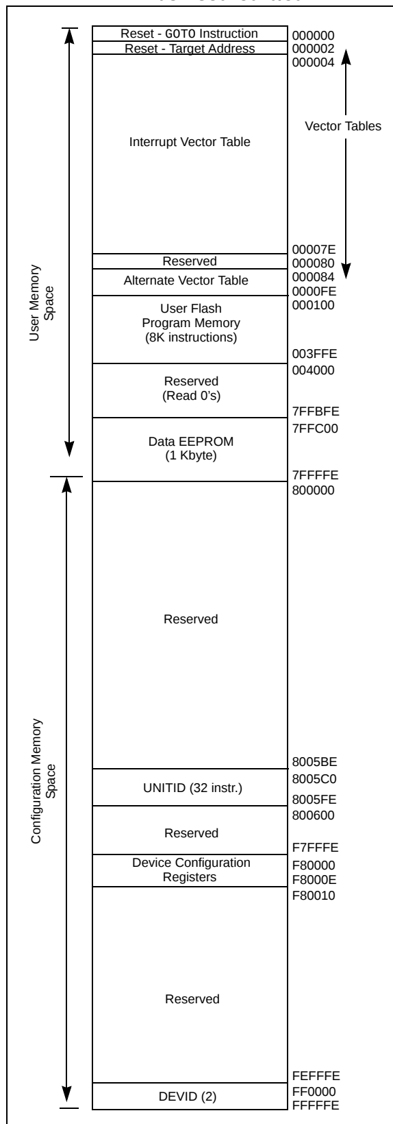
FIGURE 3-1: PROGRAM SPACE MEMORY MAP FOR dsPIC30F3010/3011
