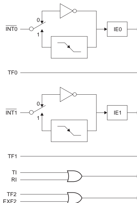
Figure 6. Interrupt Sources
