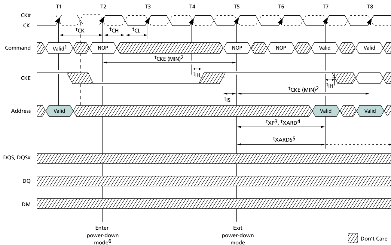
Figure 72: Power-Down
