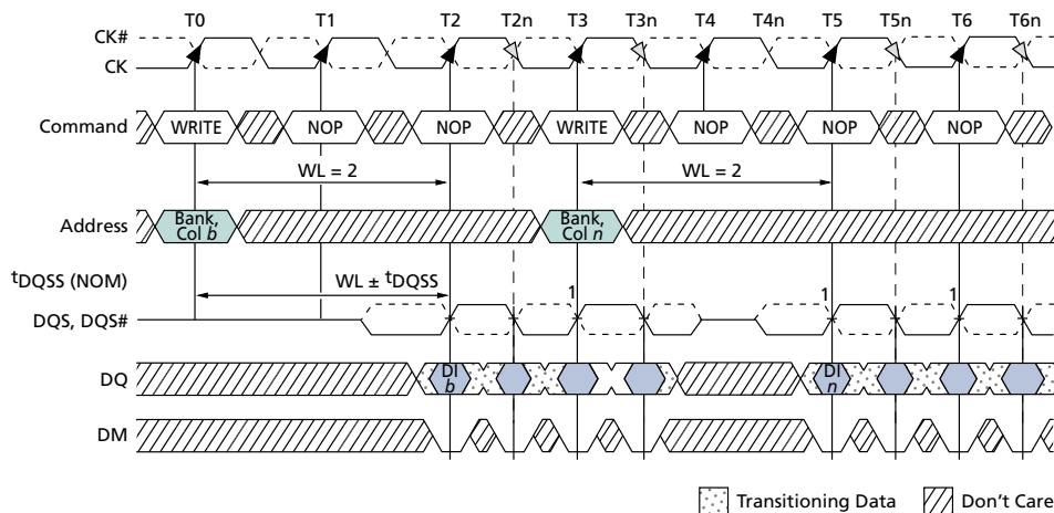
Figure 62: Nonconsecutive WRITE-to-WRITE
