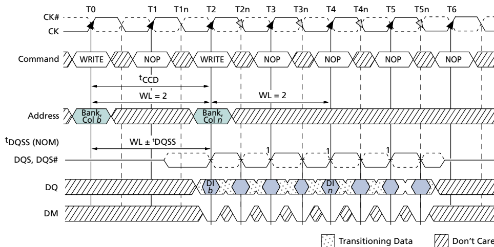
Figure 61: Consecutive WRITE-to-WRITE
