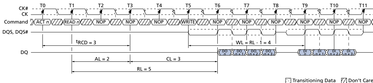
Figure 52: READ-to-WRITE
