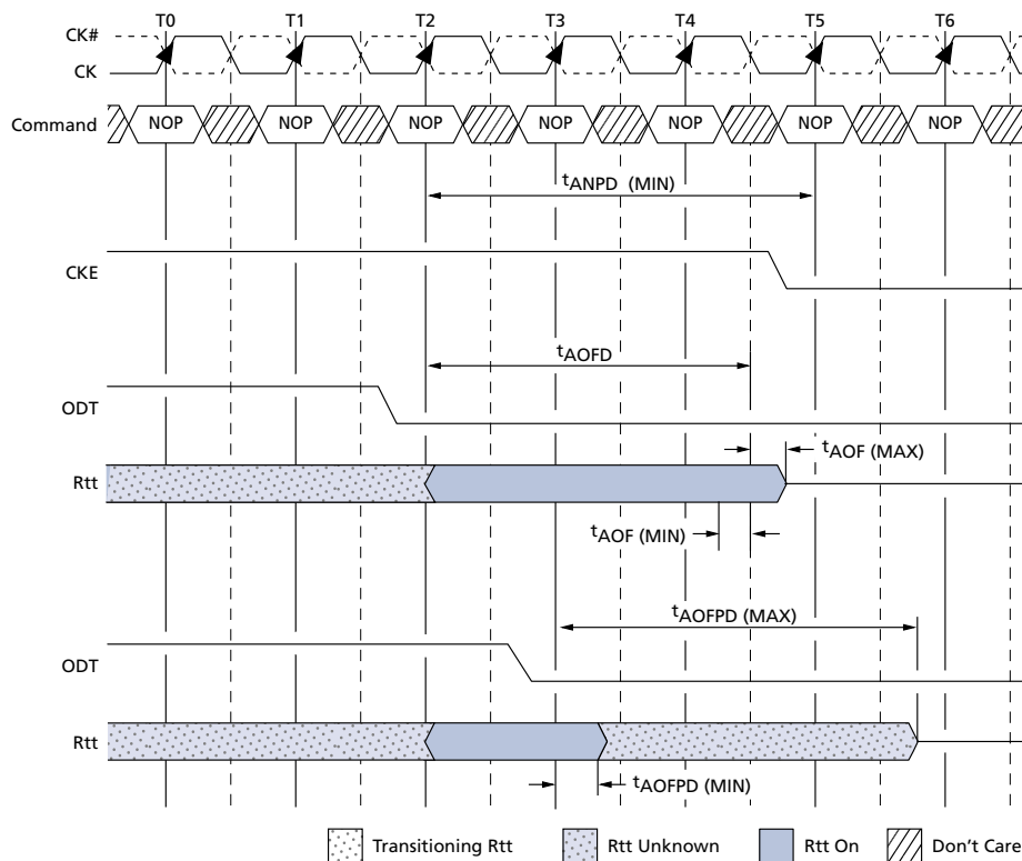
Figure 87: ODT Turn-Off Timings When Entering Power-Down Mode
