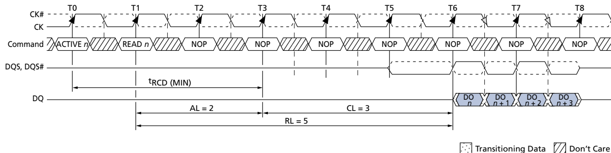
Figure 41: READ Latency
