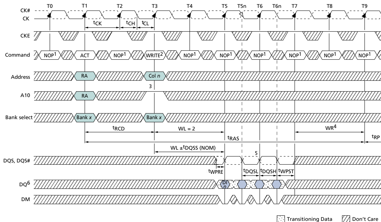
Figure 67: Bank Write – with Auto Precharge
