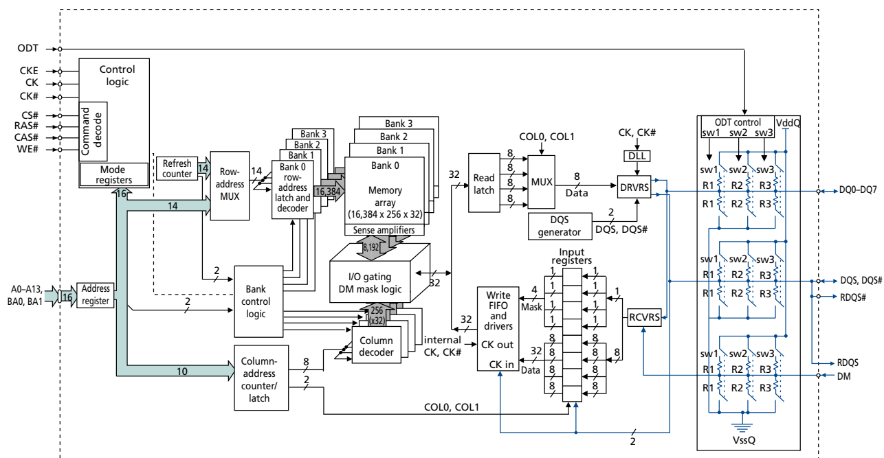
Figure 4: 64 Meg x 8 Functional Block Diagram
