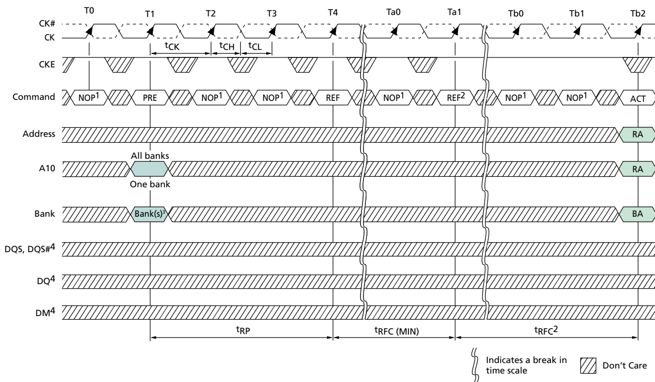
Figure 70: Refresh Mode
