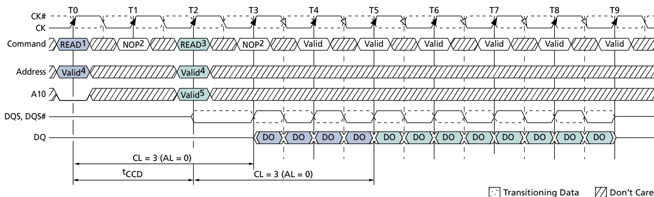
Figure 51: READ Interrupted by READ
