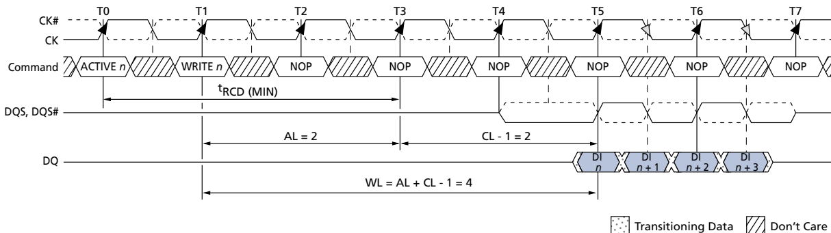
Figure 42: WRITE Latency
