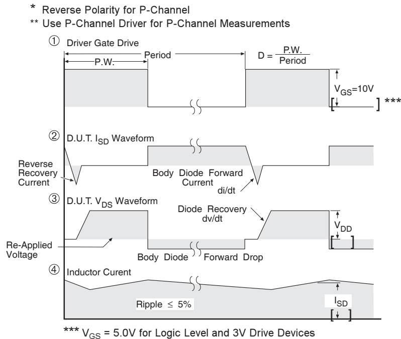
Fig 13. For P-Channel HEXFETS
