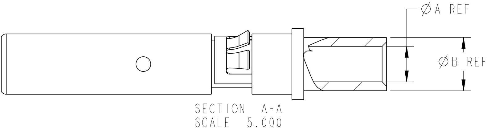
SOCKET CONTACT
