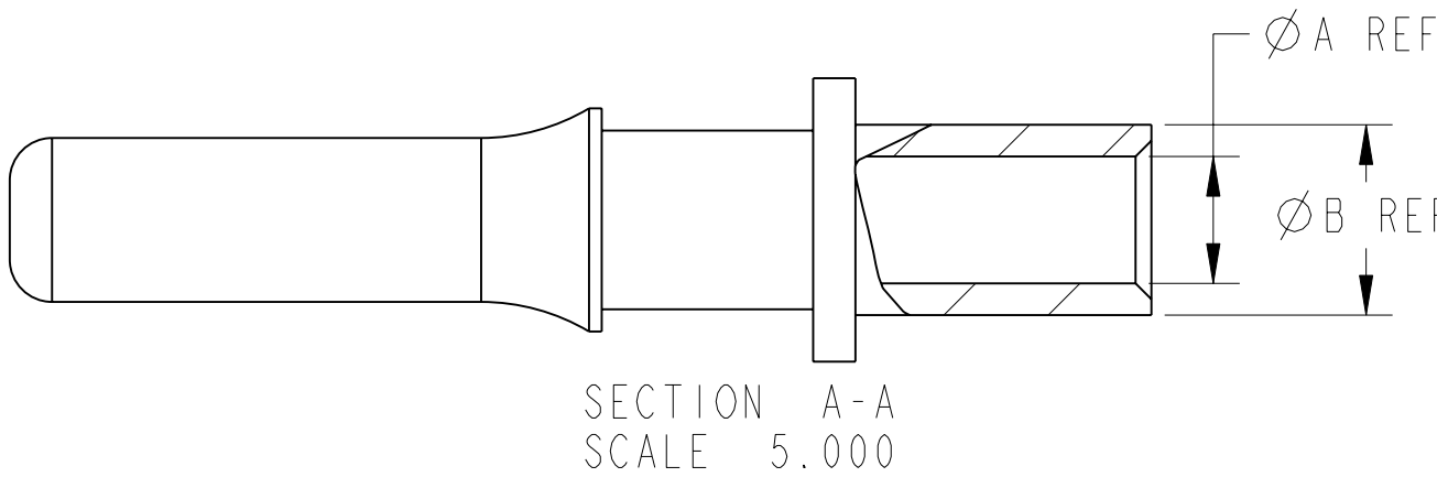
PIN CONTACT
