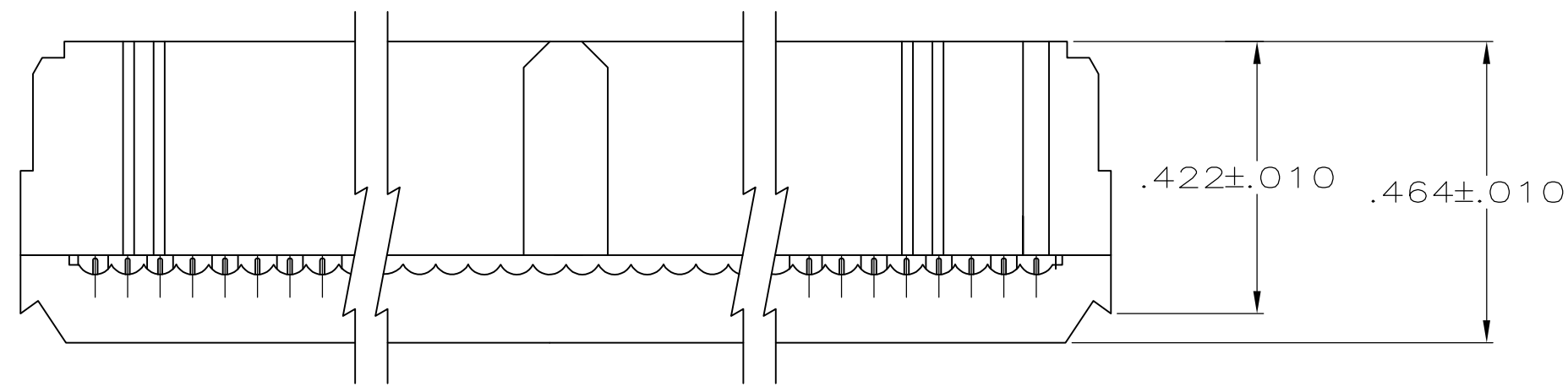
TERMINATED VIEW
