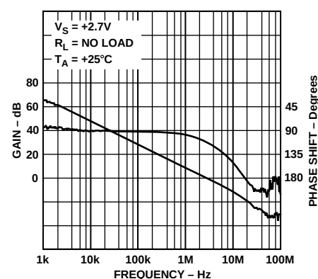
Figure 10. Open-Loop Gain & Phase vs. Frequency
