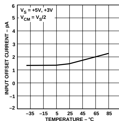
Figure 7. Input Offset Current vs. Temperature
