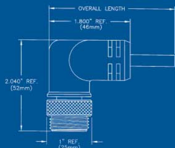
90° INLINE SINGLE-ENDED
