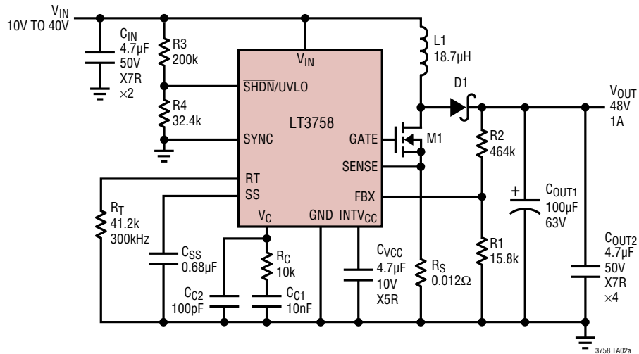
10V to 40V Input, 48V Output Boost Converter
