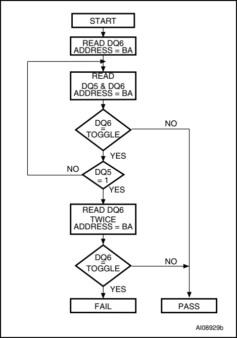
Figure 8. Toggle Flowchart
