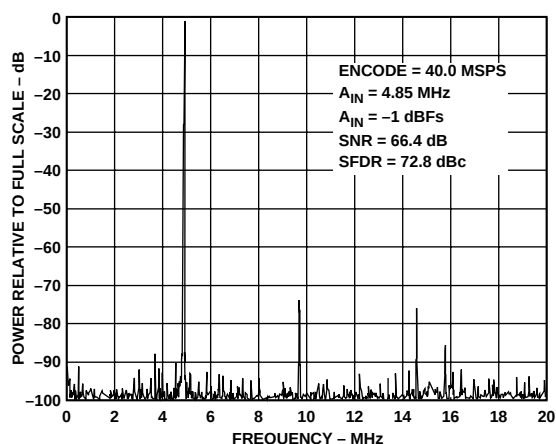
Figure 6. Single Tone @ 4.85 MHz
