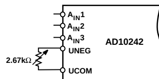
Figure 28. Unipolar Negative
