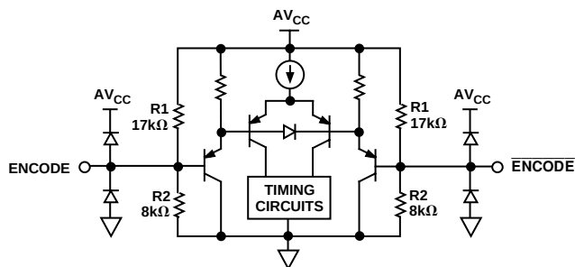
Figure 4. Encode Inputs
