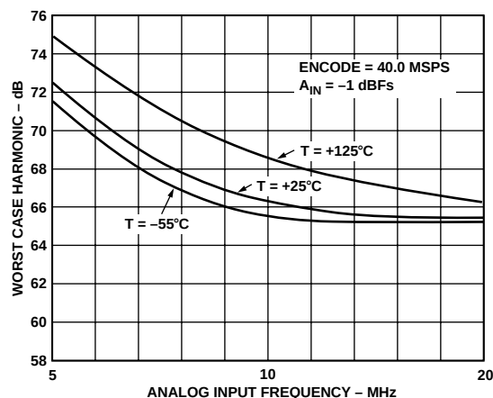
Figure 11. Harmonics vs. AIN
