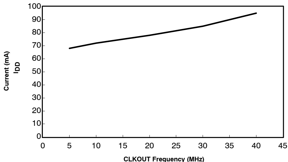
Figure 21. LF2407A Typical Current Consumption (With Peripheral Clocks Enabled)
