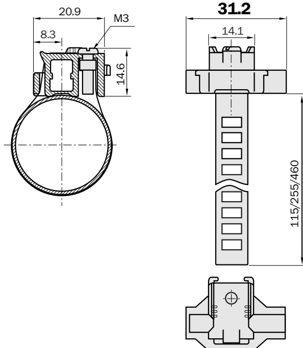
Dimensional drawing
