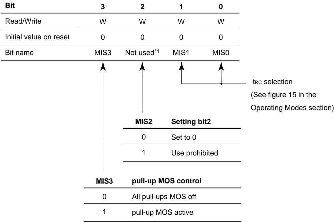
Figure 30 Miscellaneous Register (MIS:$005)
