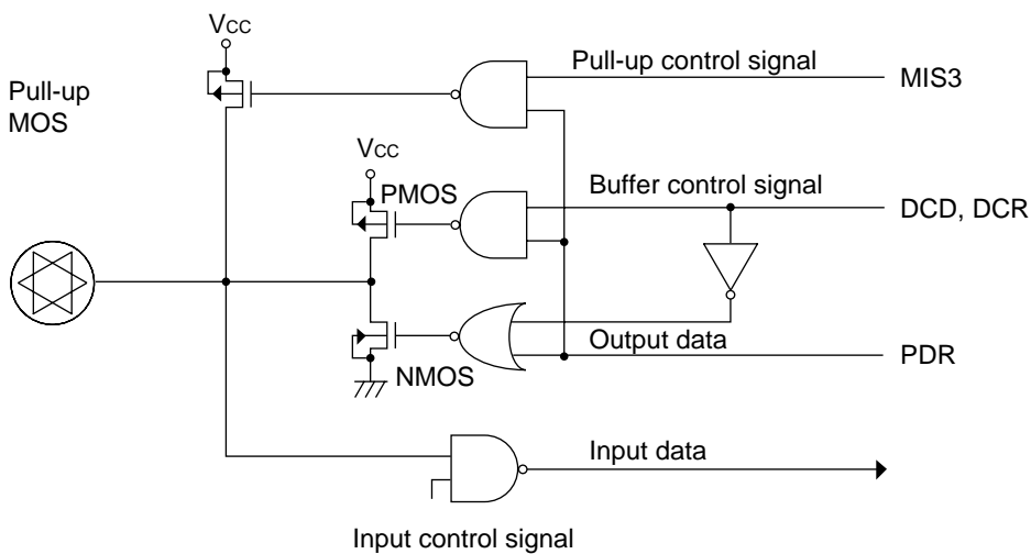
Figure 24 I/O Pin Circuit Configuration
