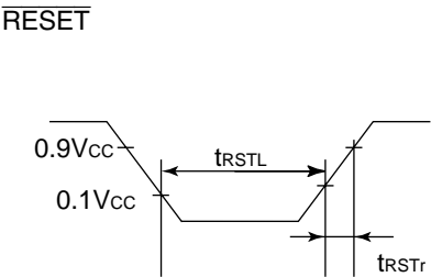
Figure 81 Reset Timing
