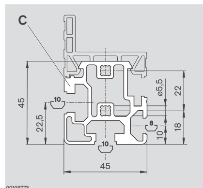
EcoFlow section profiles
