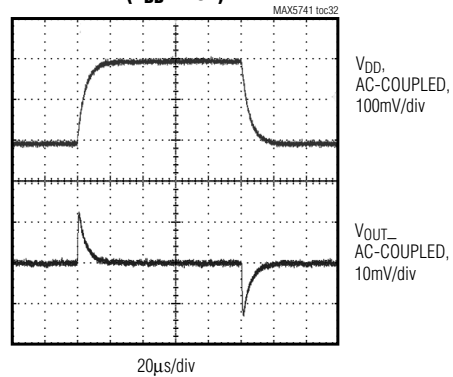
LINE TRANSIENT RESPONSE ( V_{DD} = +5V )
