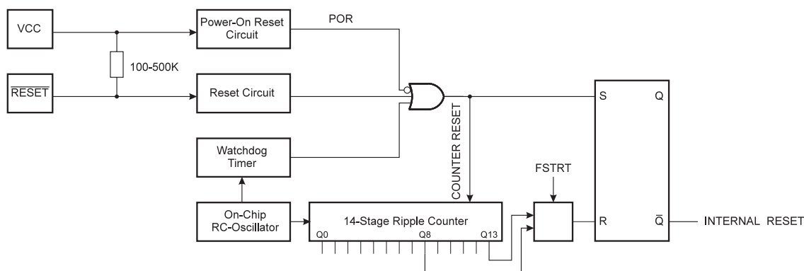
Figure 25. Reset Logic
