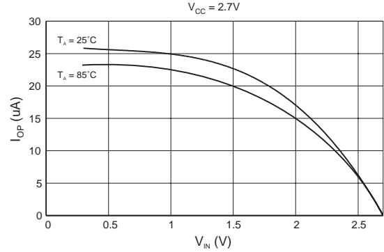
PULL-UP RESISTOR CURRENT vs. INPUT VOLTAGE
