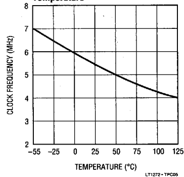
Maximum Clock Frequency vs Temperature
