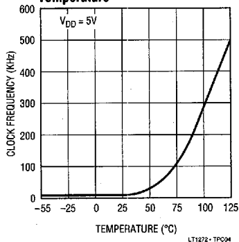
Minimum Clock Frequency vs Temperature
