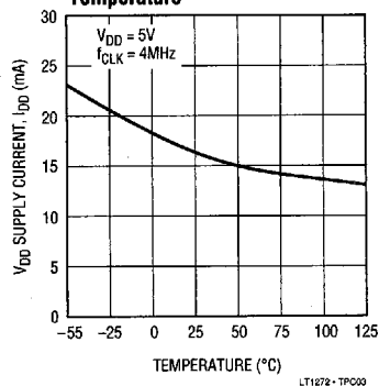
VDD Supply Current vs Temperature
