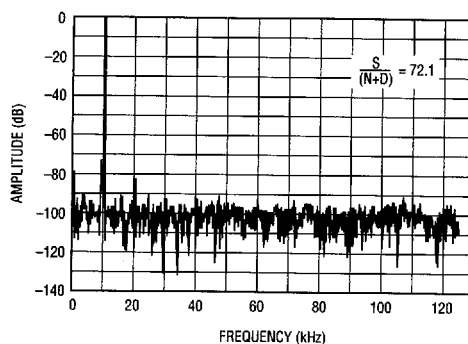
1024 Point FFT, f_s = 250\text{kHz} , f_N = 10\text{kHz}
