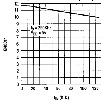
LTC1272 ENOBs* vs Frequency
