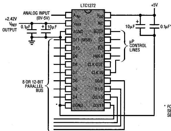
Figure 21. Single 5V Supply, 3\mu\text{s} , 12-Bit Sampling ADC
