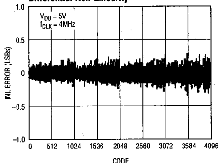
Differential Non-Linearity
