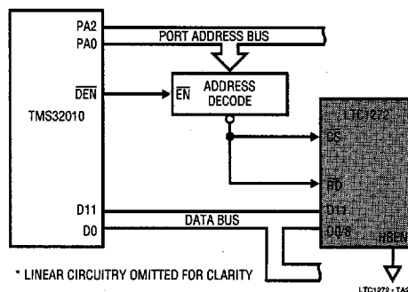
Figure 20. LTC1272 TMS32010 Interface
