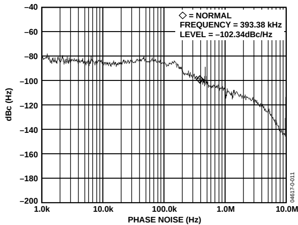
Figure 11. Phase Noise Response— I_{CP} = 2.0 mA, I_{VCO} = 2.0 mA, RF_{OUT} = 433.92 MHz, PFD = 4 MHz, PA Bias = 5.5 mA
