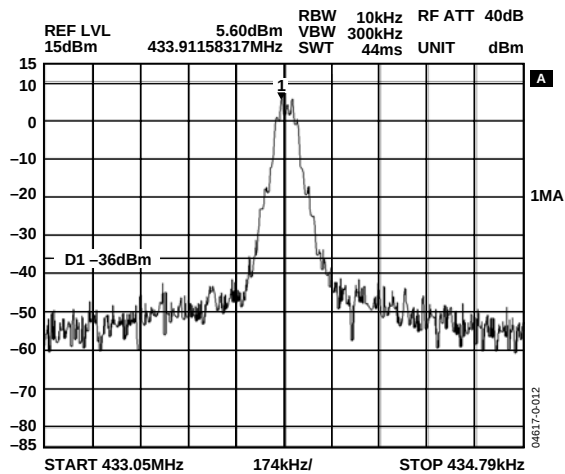
Figure 11. Phase Noise Response— I_{CP} = 2.0 mA, I_{VCO} = 2.0 mA, RF_{OUT} = 433.92 MHz, PFD = 4 MHz, PA Bias = 5.5 mA
