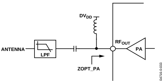
Figure 38. ADF7012 with Harmonic Filter
