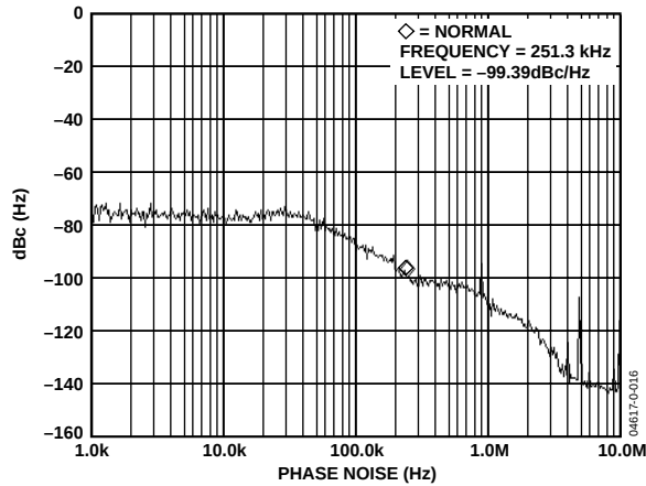
Figure 16. Phase Noise Response— I_{CP} = 2.5 mA, I_{VCO} = 1.44 mA, RF_{OUT} = 868.95 MHz, PFD = 4.9152 MHz, Power = 12.5 dBm, PA Bias = Max
