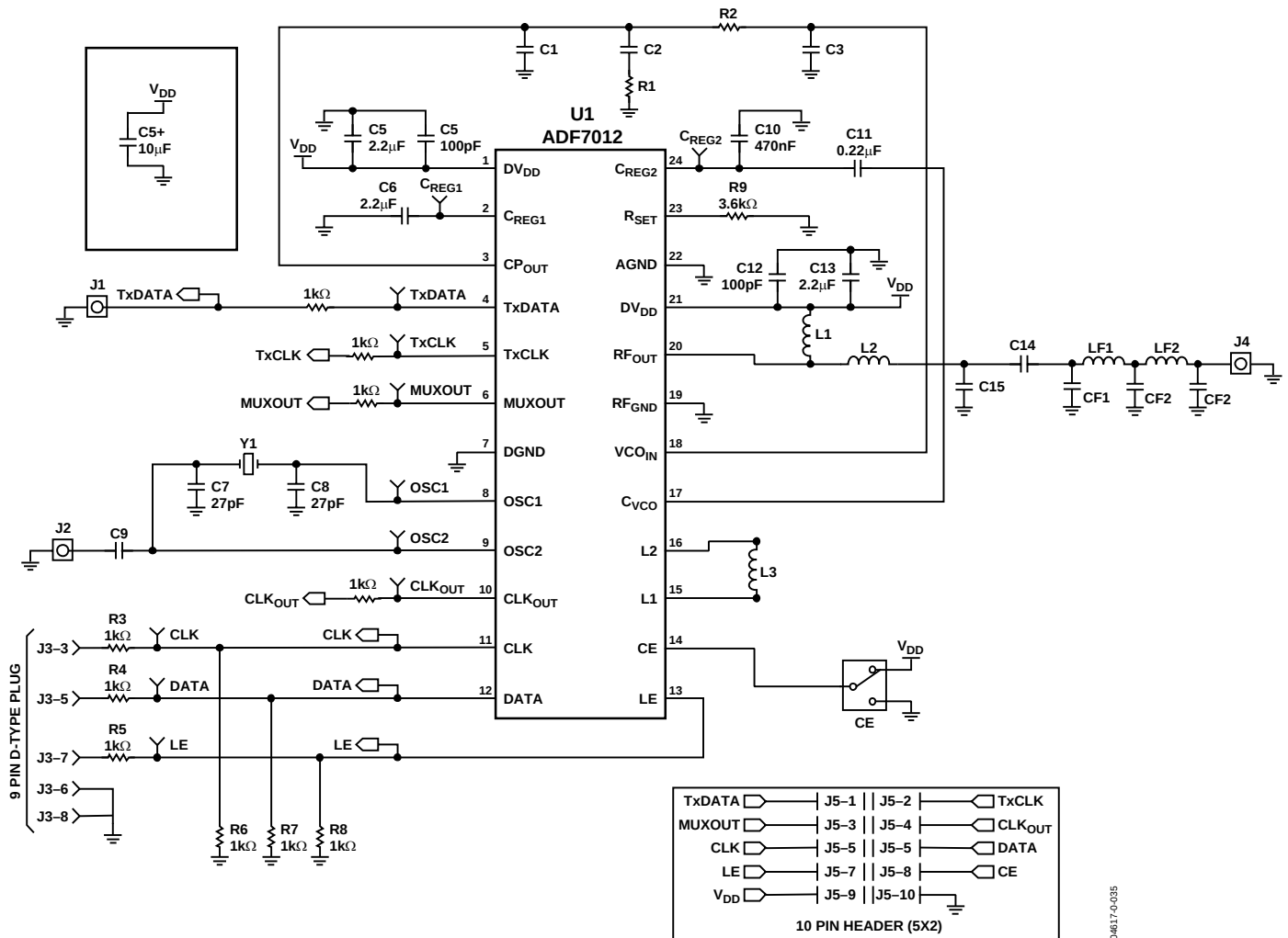
Figure 40. Applications Diagrams with Harmonic Filter
