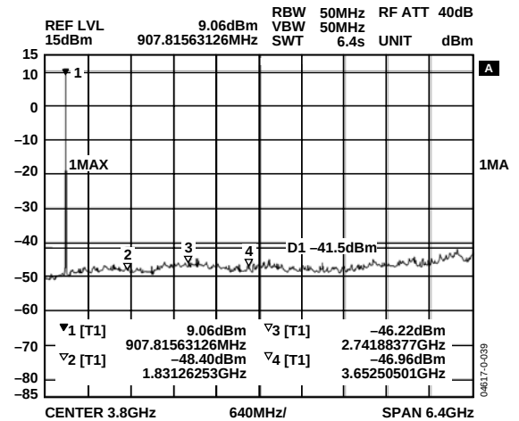
Figure 25. Harmonic Response, Fifth-Order Chebyshev Filter
