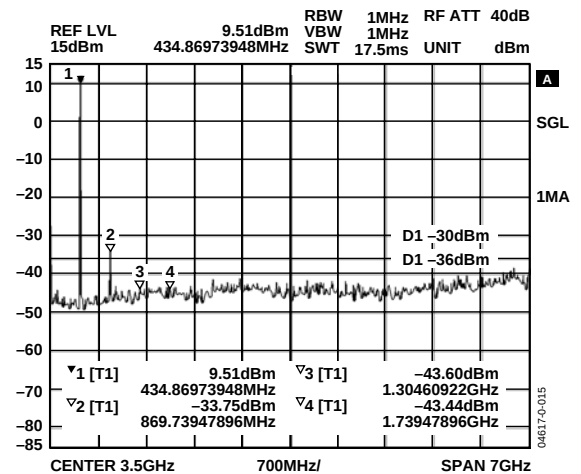
Figure 15. Harmonic Response, Fifth-Order Butterworth Filter
