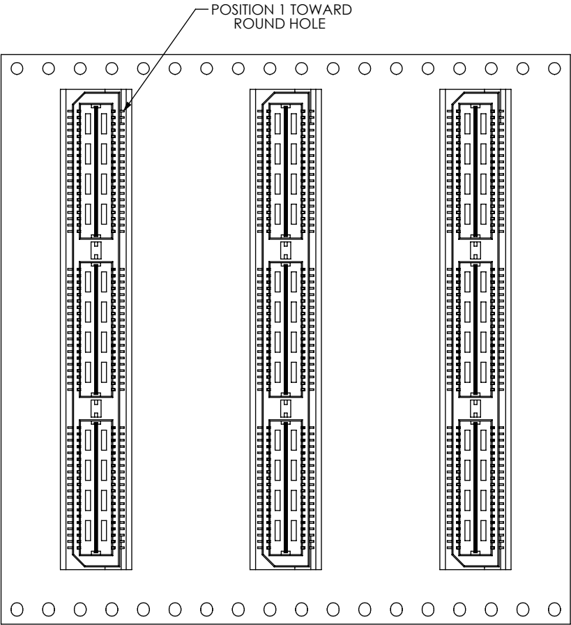
FIG 10 -TR: PACKAGING OPTION (NOT AVAILABLE ON LEAD SYTLES -05, -06, -07 & -08) (SAME AS FIG 1, UNLESS OTHERWISE STATED)
