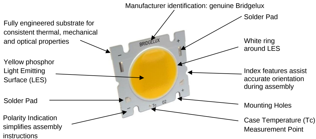
Figure 1: Array Features
