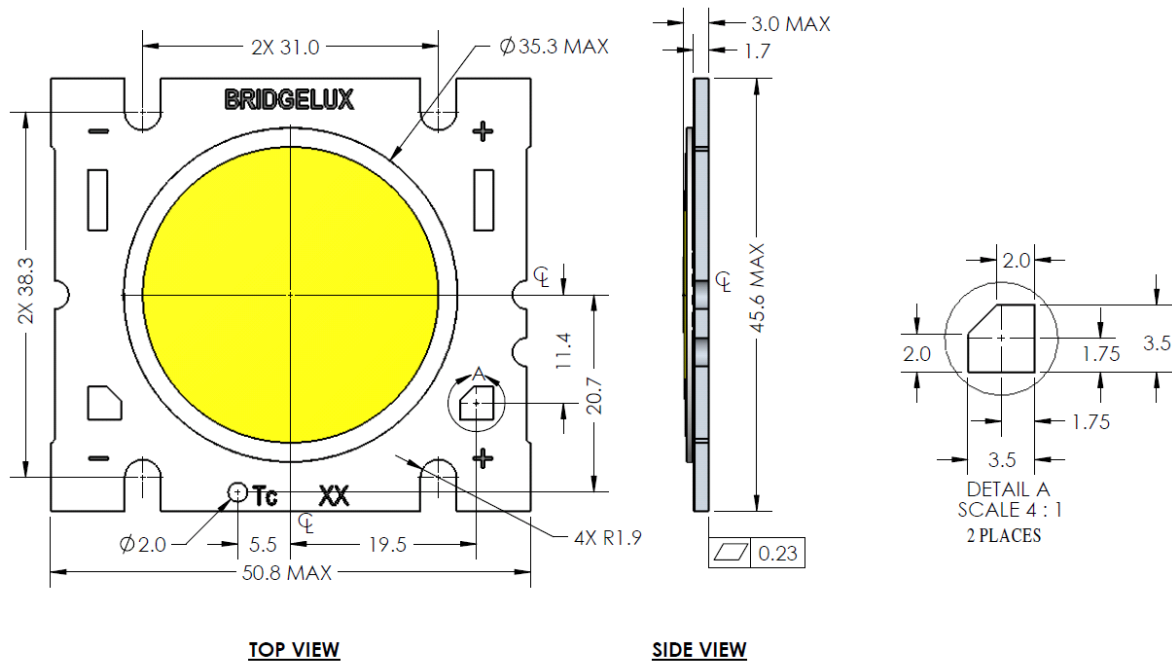
Figure 14: Drawing for RS Arrays
