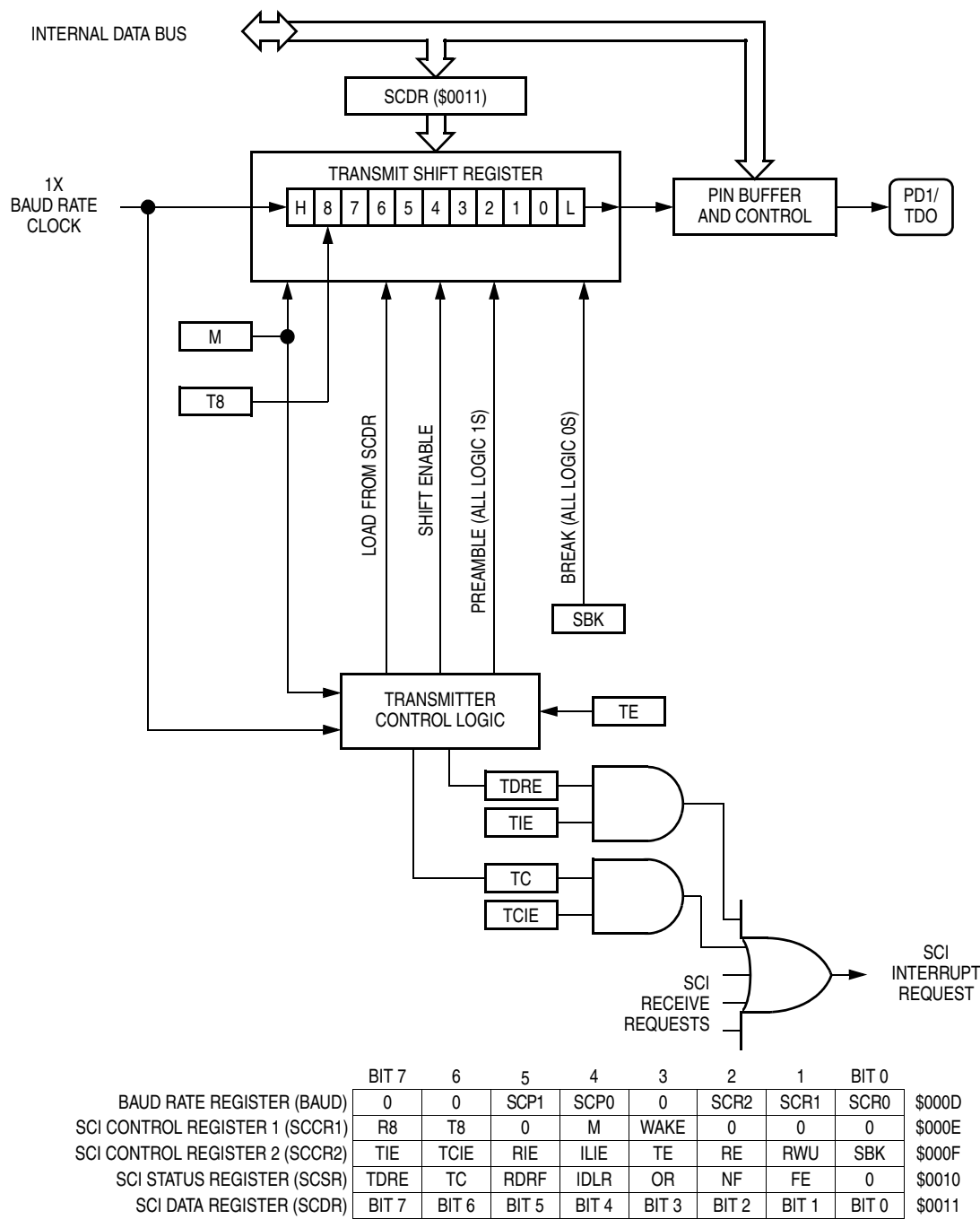
Figure 9-2. SCI Transmitter
