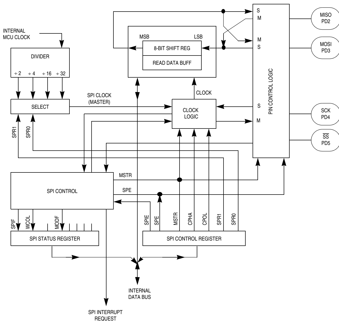
Figure 10-2. Serial Peripheral Interface Block Diagram
