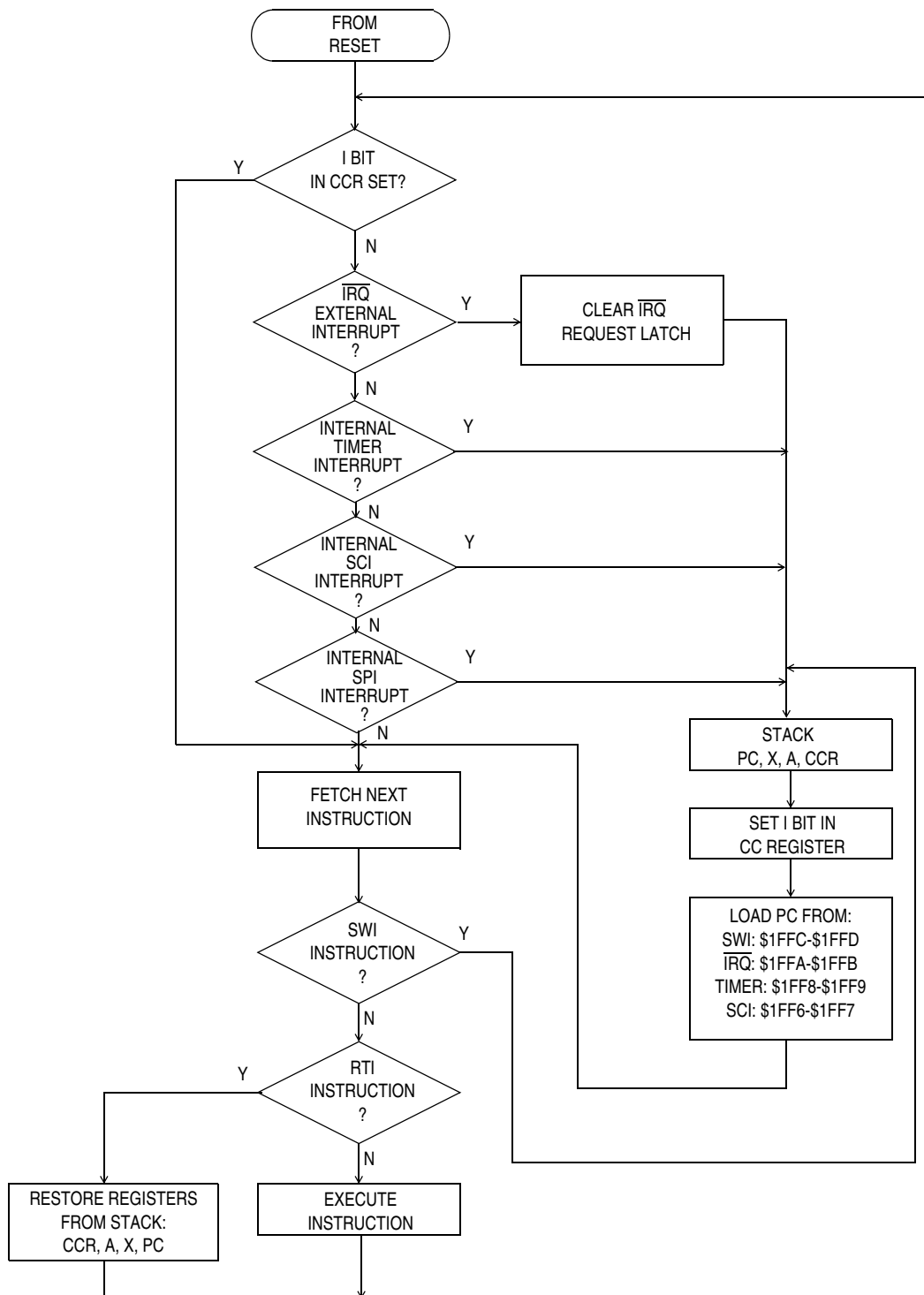
Figure 4-1. Interrupt Flowchart
