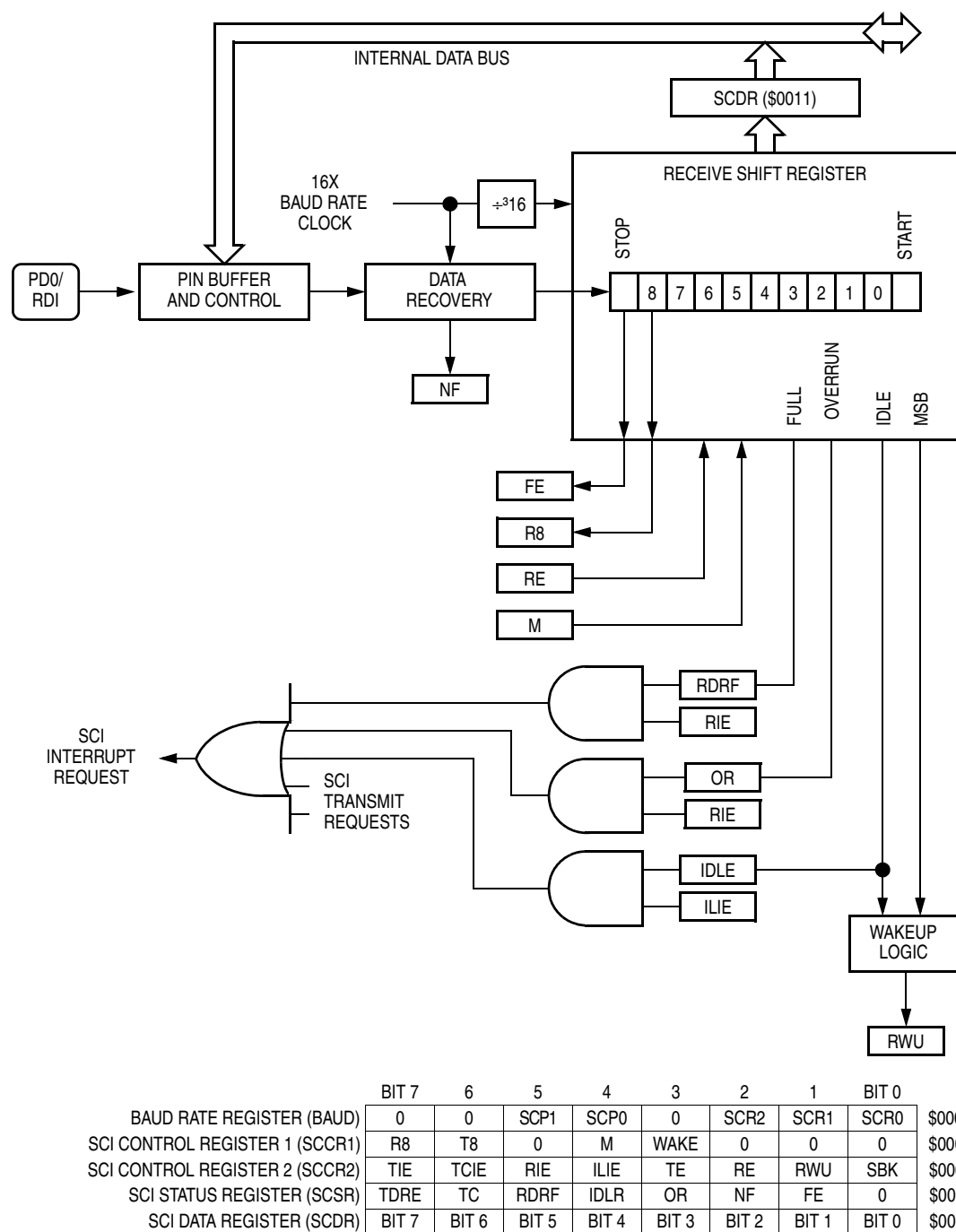
Figure 9-3. SCI Receiver
