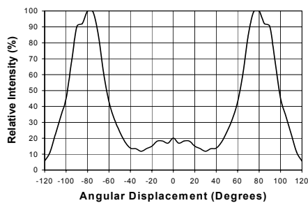
Figure 8a. Representative Spatial Radiation Pattern for Luxeon Emitter Red and Amber
