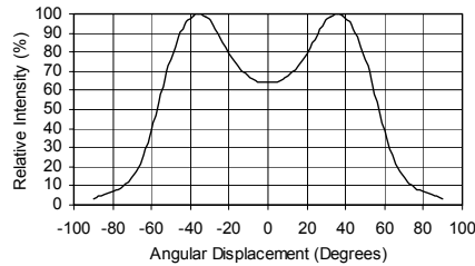
Figure 6a. Representative Spatial Radiation Pattern for Luxeon Emitter White.
