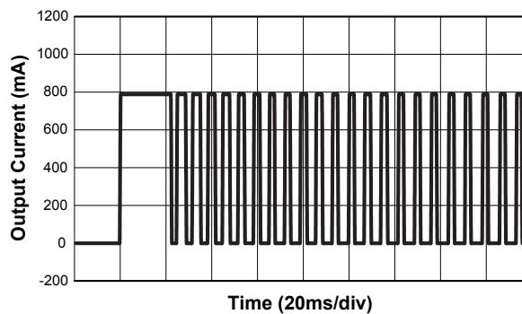
Over-Current Protection
