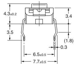
PCB Mounting (Top View) (Single-sided PCB, t=1.6)
