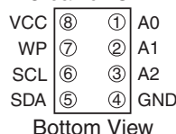
8-lead SOIC
