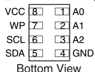
8-lead TSSOP
