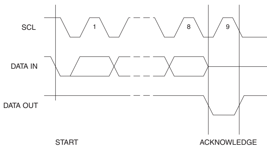
Figure 5-4. Output Acknowledge
