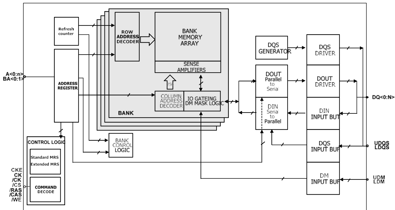
Figure.2 — Block Diagram
