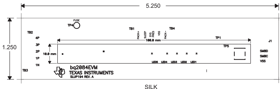
Figure 2. bq2084EVM-001 Layout
