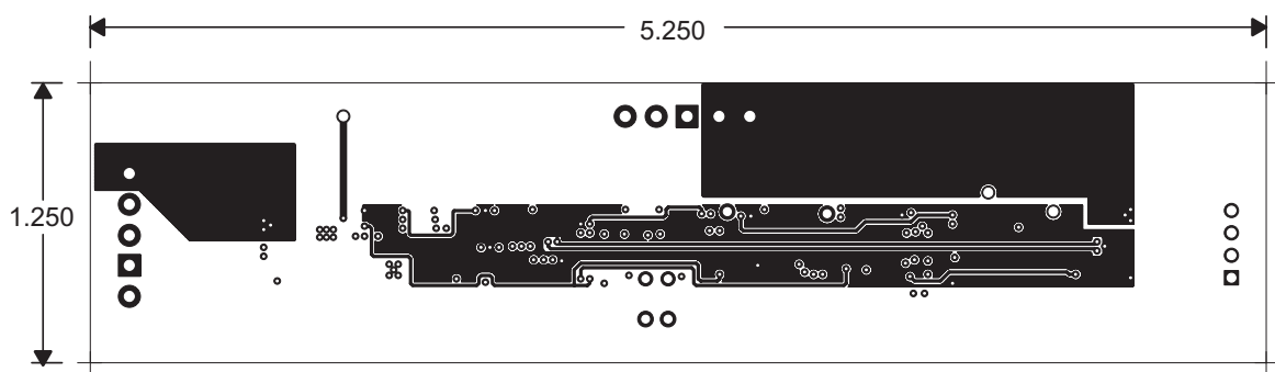
LAYER 2 [ INTERNAL 1 ]
