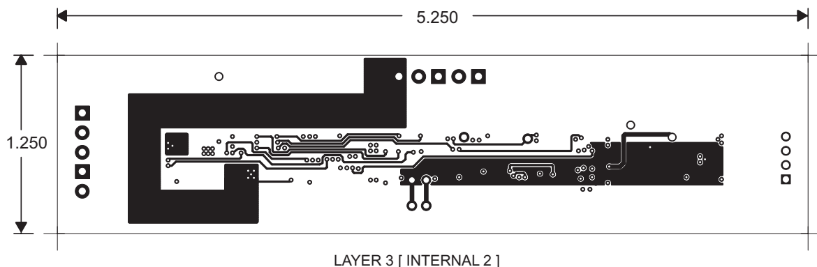
Figure 6. Layer 3 (Internal 2)
