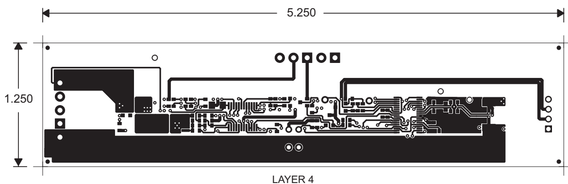
Figure 7. Layer 4
