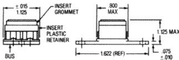
Type K: Flange Mount
