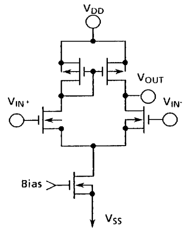
Figure 18 Comparator
