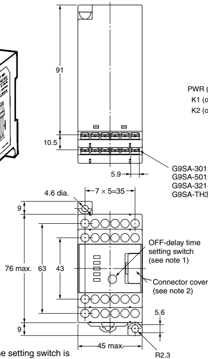
G9SA-301
