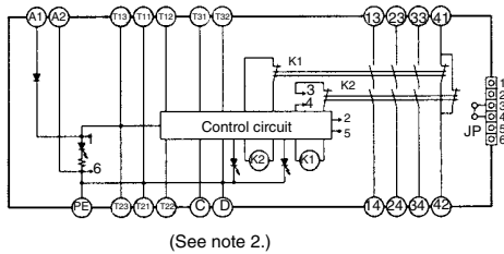
G9SA-EX301
