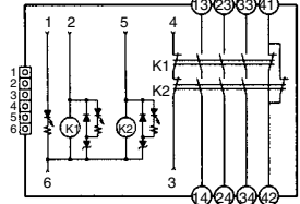
G9SA-EX031-T
