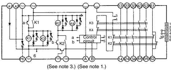
G9SA-321-T (24 VAC/VDC)
