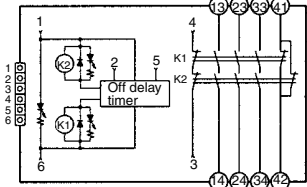
G9SA-EX031-T
