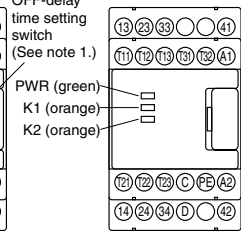
G9SA-TH301
