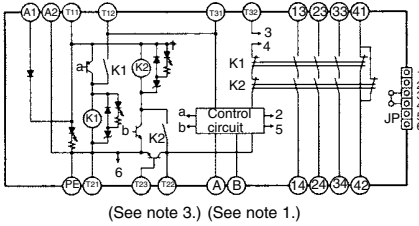
G9SA-501 (24 VAC/VDC)
