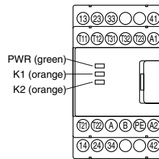
G9SA-301
