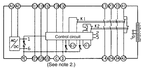
G9SA-TH301 (100 to 240 VAC)
