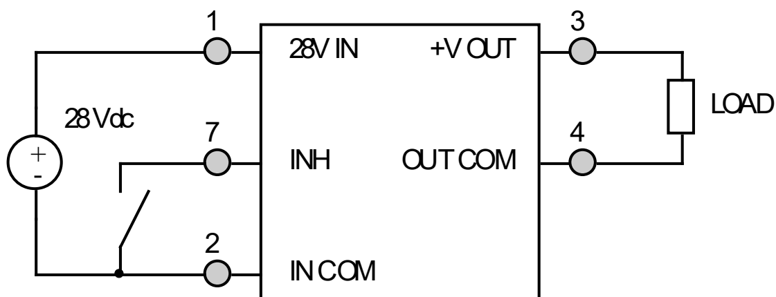
CONNECTION DIAGRAM
