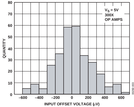
Figure 3. OP183 Input Offset Voltage Distribution @ \pm 15 V
