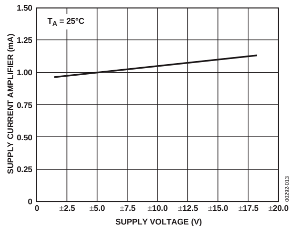
Figure 13. Supply Current per Amplifier vs. Supply Voltage
