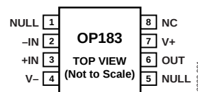
Figure 1. 8-Lead Narrow Body SOIC (S Suffix)
