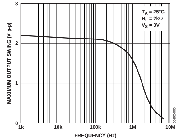
Figure 6. OP183 Maximum Output Swing vs. Frequency @ 3 V
