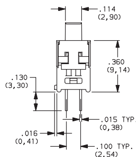
ES02 Models: omit terminal 2.
