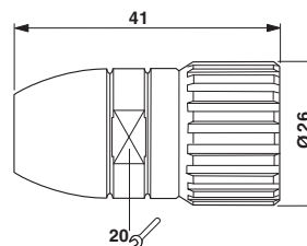
Dimensioned drawing
