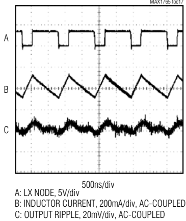
LIGHT-LOAD SWITCHING WAVEFORMS (V IN = +2.4V, V OUT = +3.3V, I OUT = 10mA)
