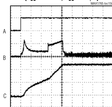
SOFT-START WAVEFORMS ( R_{SS} = 500\text{k}\Omega , C_{SS} = 0.1\mu\text{F} )
