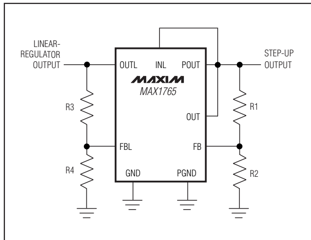
Figure 7. Feedback Connections
