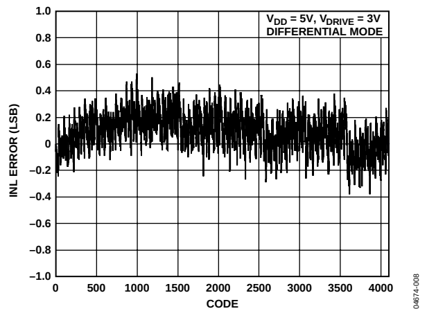
Figure 9. Typical INL
