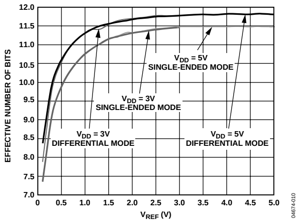
Figure 11. ENOB vs. V_{REF}
