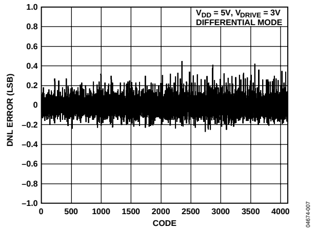
Figure 8. Typical DNL
