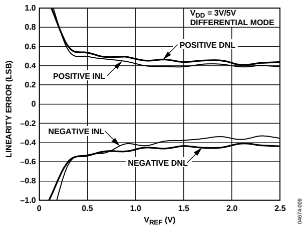
Figure 10. DNL vs. V_{REF}
