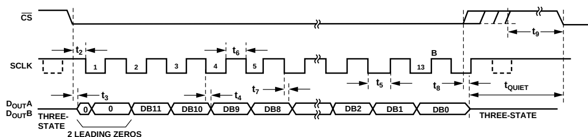
Figure 41. Serial Interface Timing Diagram
