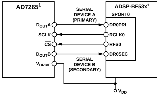
Figure 44. Interfacing the AD7265 to the ADSP-BF53x
