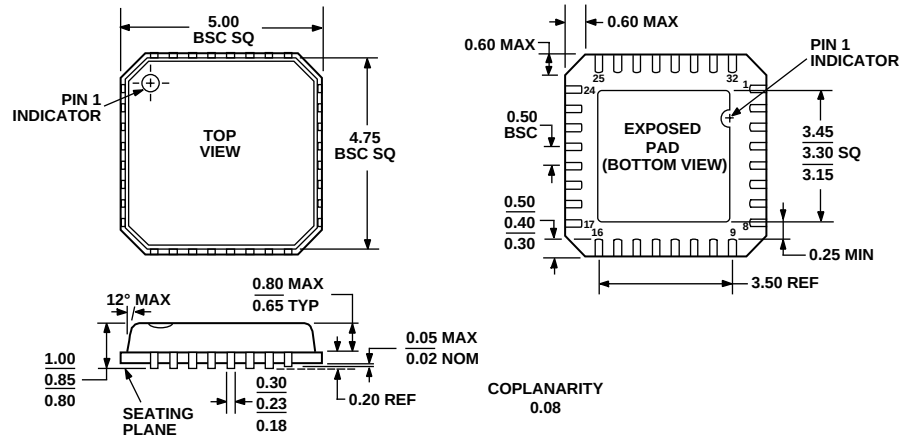
Figure 47. 32-Lead Lead Frame Chip Scale Package [VQ_LFCSP] 5 mm x 5 mm Body, Very Thin Quad (CP-32-3) Dimensions shown in millimeters
