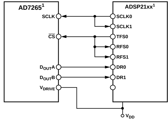
Figure 43. Interfacing the AD7265 to the ADSP218x
