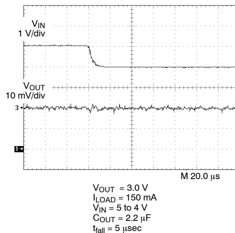
Line Transient Response-2
