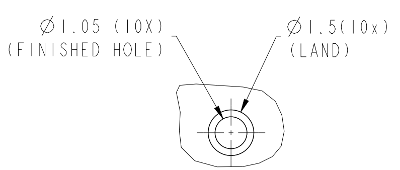
DETAIL C SCALE 8:1 SHIELD HOLES
