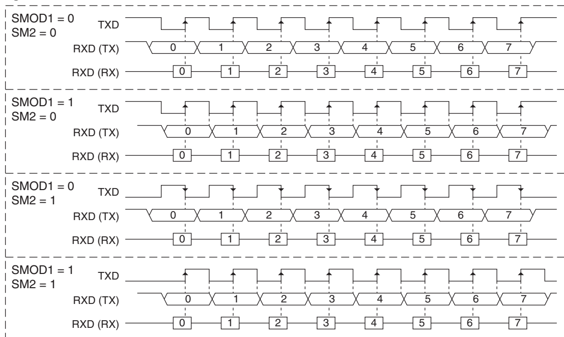
Figure 16-2. Mode 0 Waveforms
