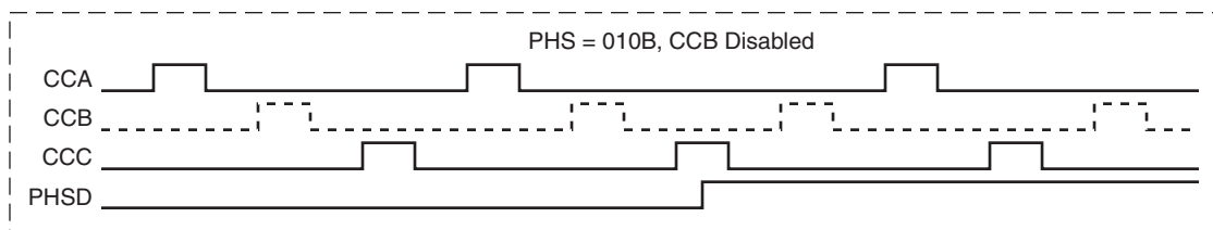
Figure 13-14. Three-Phase Mode with Channel B Disabled
